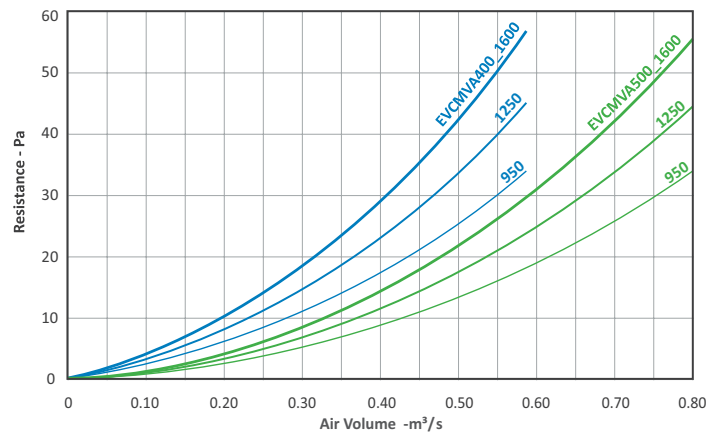
Performance curves
